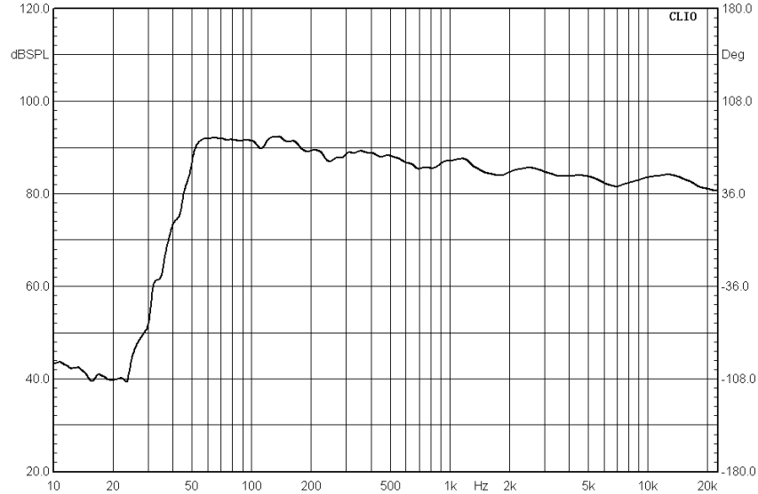
Curve of Pro5 V3 speaker (dB SPL, resolution 1/12 d'octave):
