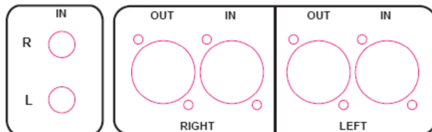
Figure 9 – TRS, XLR inputs/outputs for the Pro10SV3 Subwoofer
